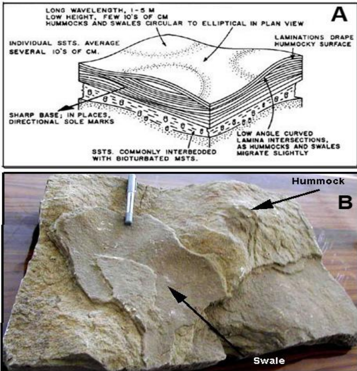
Fig.3A: Comparison between sketch of hummocky cross stratification by Walker(1984) and B: Photo of hummocky cross stratification structure found at Dokan area near Joblagh village, 2km east of tourism camp. One can observe the parallelism of the lamina covering the surface of hummock and swale.
