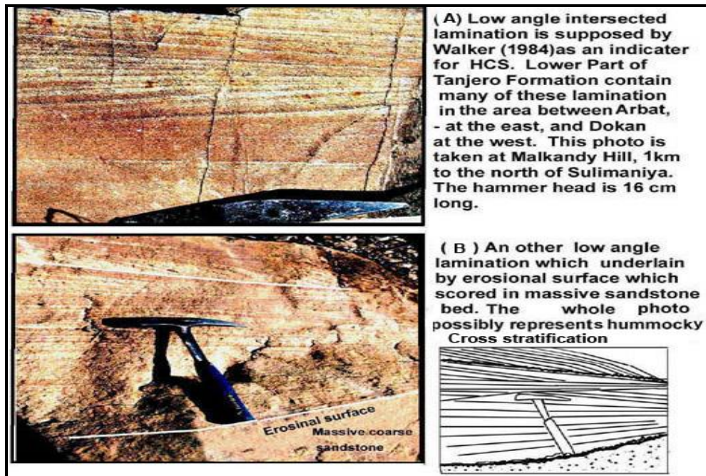
Fig. 5: Low angle cross lamination (A and B) found in the sandstone of Tanjero Formation possible represent part of hummocky cross stratification with their description at right side.
