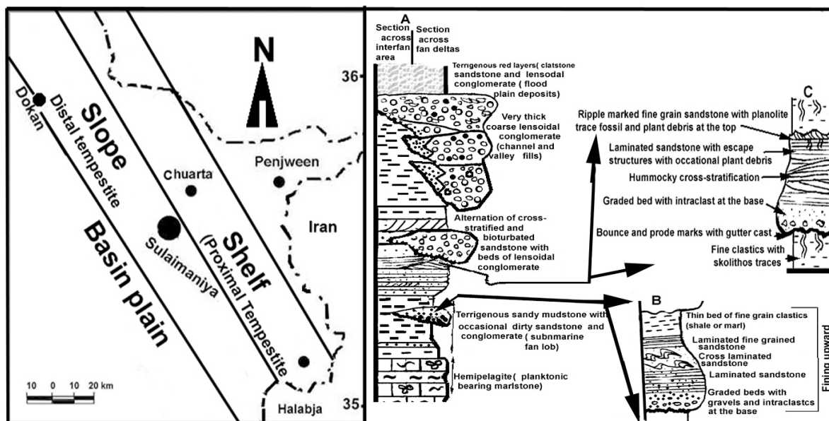
Fig. 2 Left: Position of shelf, slope and basin plain of Tanjero Formation during lowstand system tract. The position of proximal and distal tempestite is indicated. Right: A) General Facies model for the formation, B) facies model for turbidite, C) Facies model for tempestite.
