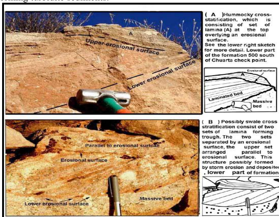
Fig.7: Sedimentary structures supposed to be formed by storm found in the sandstone succession of the lower part. The descriptions of each photo are given at right side with graphic sketch of each one.
