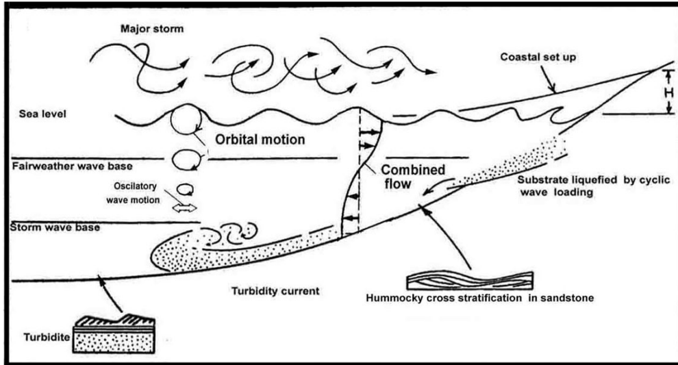
Fig. 4: Storm dominated shelf (Walker, 1984) used to illustrate the possibility of deposition of tempestite and turbidite by storm in shallow and deep part of the same basin.
