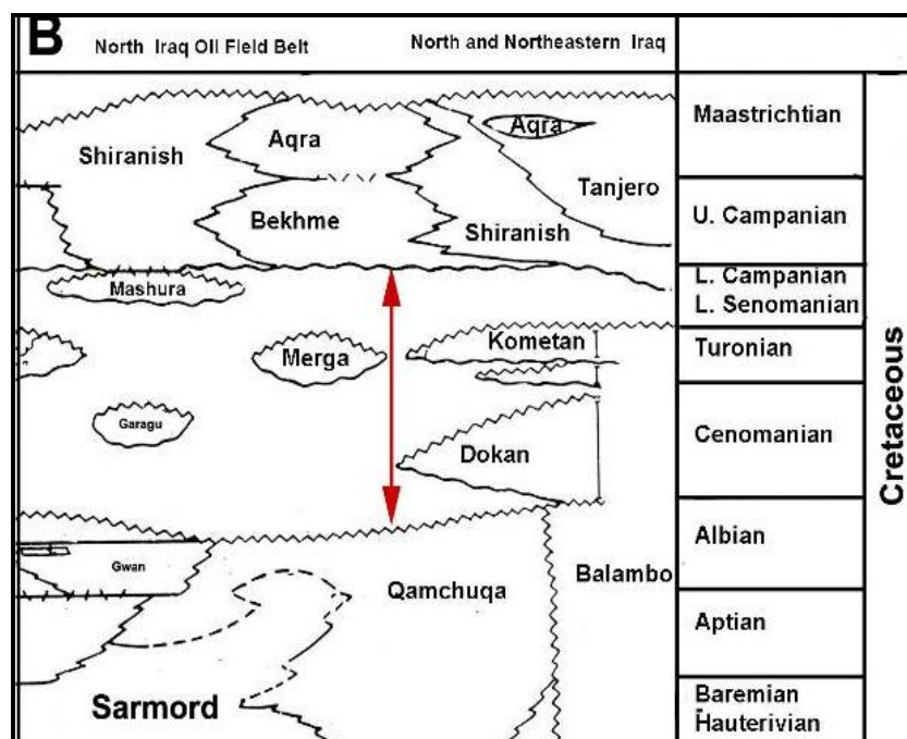
Fig. (11) The time expanded stratigraphic column of Northern and Northeastern Iraq shows the position and extent of the gap of the unconformity (Bellen et al., 1959).
