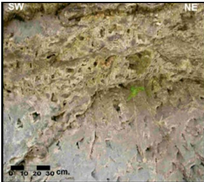
Plate ( 2-3) Basal conglomerate 4m thick between Qamchuqa and Bekhme Formations in Perat anticline contain clasts of limestone of Qamchuqa Formation
