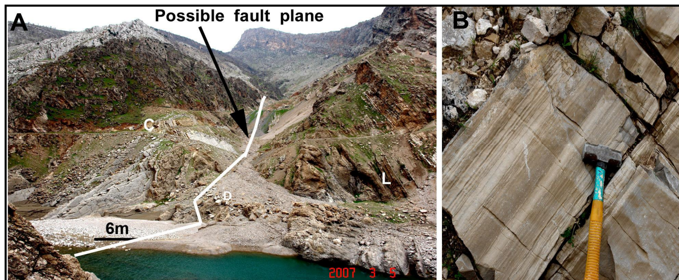
Fig.4: A) Boundary between Qamchuqa and Aqra–Bekhme formations at Bekhme inlet (according to stream flow direction) showing location of Ball and pillow-like structures(C), breccias (D). The trace of possible reverse fault is indicated across the valley surface by white line. B) The close up photo of laminated limestone beds (L).
