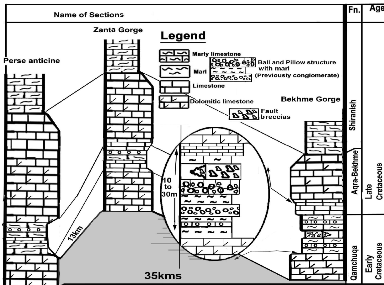
Fig.2: Conformable boundary between Qamchuqa and Aqra-Bekhme formations at three different sections in Bekhme and Zante gorges and Perse anticline.
