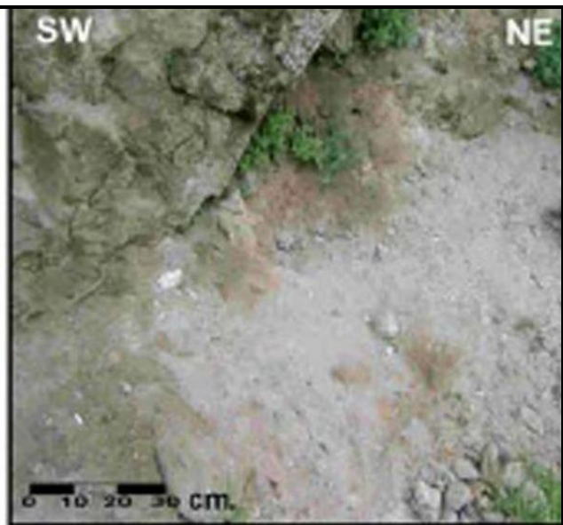
Plate( 2-4) contact between the two formations in the Shakrok anticline composed of Saccharoidal dolomite nearly 5-6m thick
