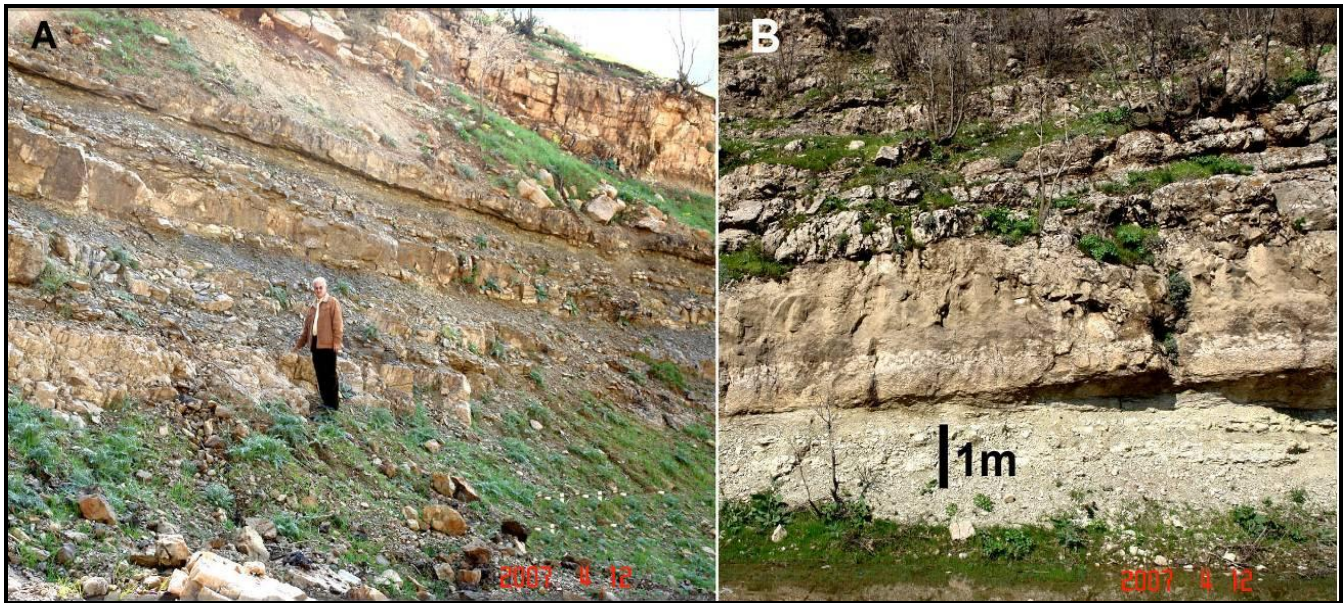
Fig.8: Boundary between Qamchuqa and Bekhme Formations at southwestern and northeastern upper limb of Perse anticline at northeast of Dinarta town. The boundary consists of intercalation of marl and bioturbated dolomitic limestone, which is possibly gradational.
