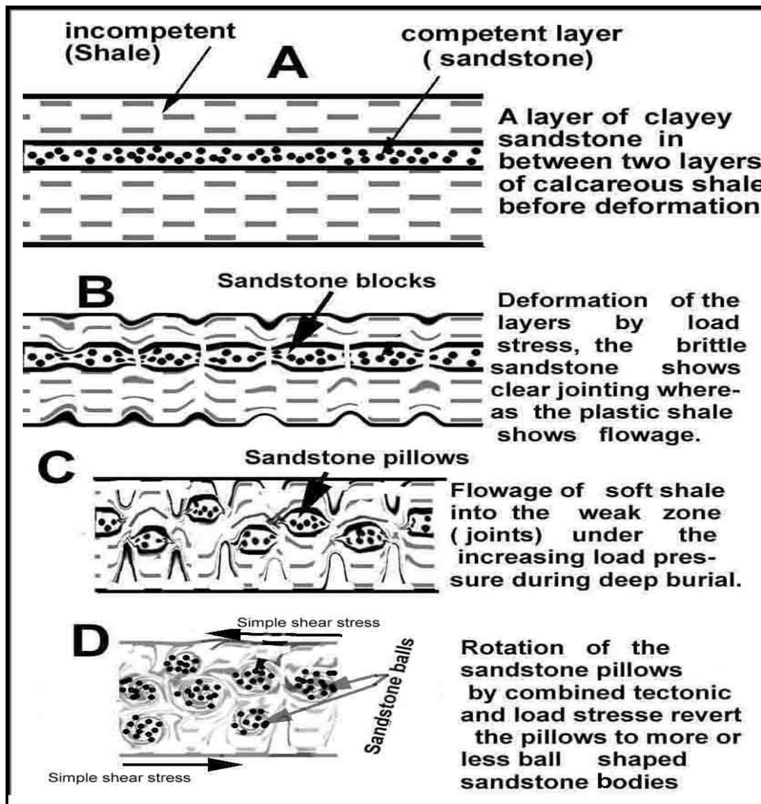
Fig.6: Four stages of development of ball and pillow structure by tectonic stresses when competent and incompetent beds are associated (Karim, 2006).
